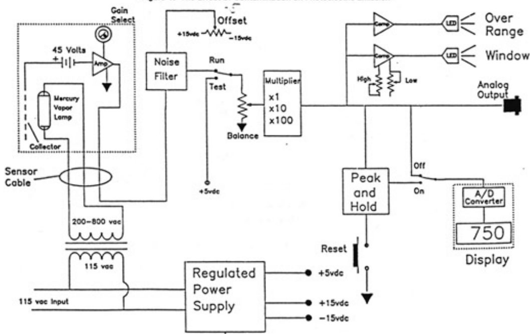
Figure 2. OSEE Monitor Block Diagram
