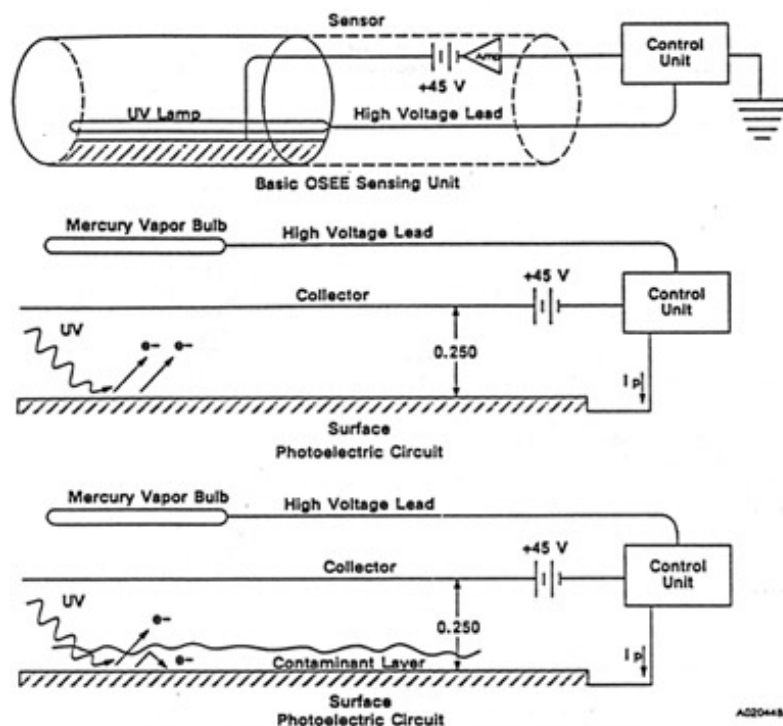
Figure 1. The Effect of Contamination on Photoelectric Emission
