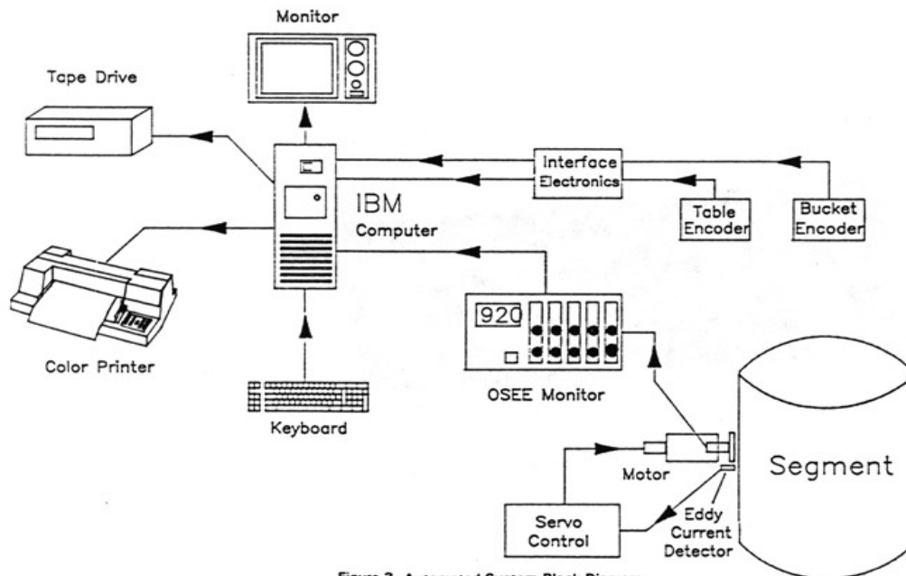
Figure 3. Automated System Block Diagram
